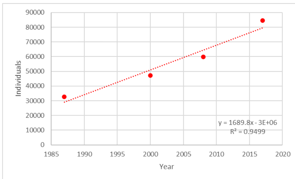
Plate 7-1: Guillemot Counts (Individuals) at the FFC SPA between 1986 and 2017 Included in the Seabird Monitoring Programme (SMP) Database (JNCC, 2022), with Linear Trendline. Note That These Values Have Not Been Corrected to Estimate the Number of Birds Not at the Colony at the Time of the Count, so Do Not Match the Values Given in the Text.
